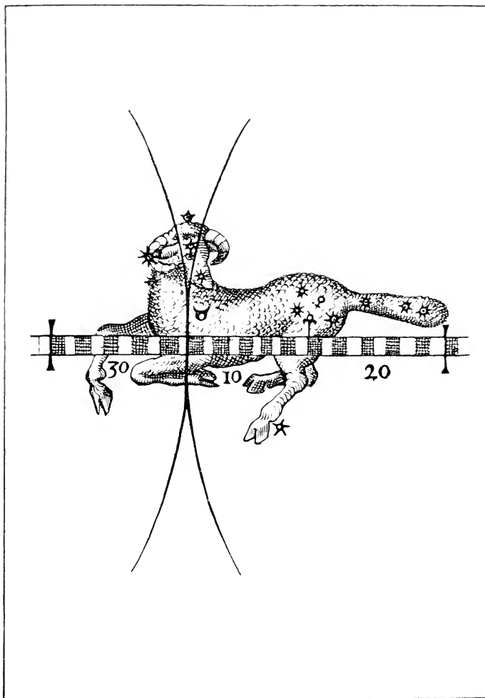
Fig. 41. The Ram on the Ecliptic. [To face p. 279. From the "Cosmi Historia" of Robert Flud, A.D. 1612. (Reproduced from Brown's Phainomena of Aratos. )
